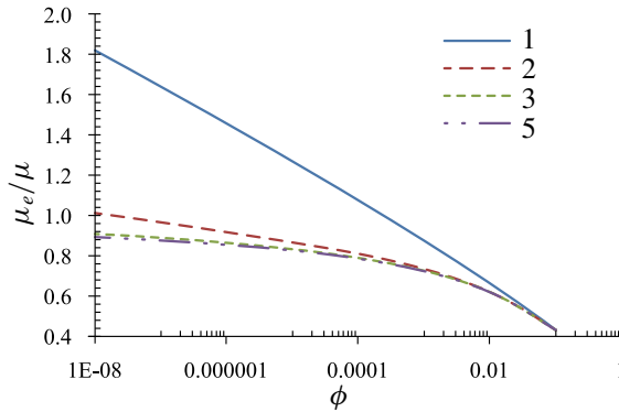
Figure 8. Influence of the number of the rows of fibers \{1, 2, 3, 5\} for the square array on the values of the dimensionless effective viscosity \alpha for different values of the volume fraction \phi .
