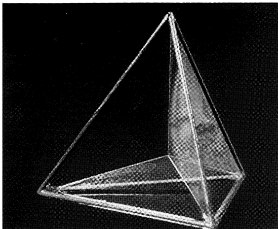
FIGURE 1.0.1. The cone over the tetrahedron provides the least-area soap film which separates the four regions. Photo by F. Goro.
