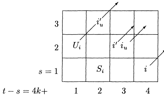
Figure 1.7: v_1^{-1}E_2^{s,t}(S^{4i-1})
