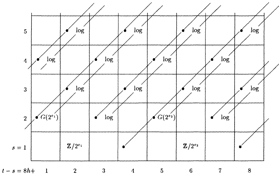
Figure 1.16: v_1^{-1}E_2^{s,t}(Sp(n))
