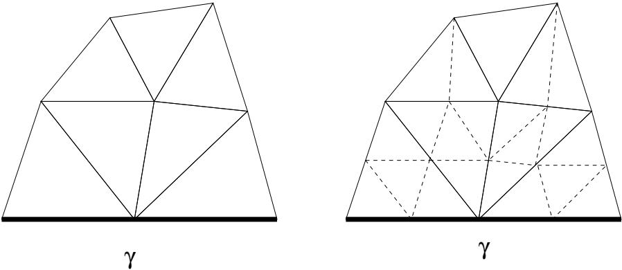
Figure 8. A complex (left) can be locally hex refined along an edge path \gamma (right).
