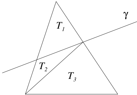
Figure 10. Adding an edge corresponding to \gamma , we form a triangle T_1 and a quadrilateral. A second edge then breaks the quadrilateral into triangles T_2 and T_3 .
