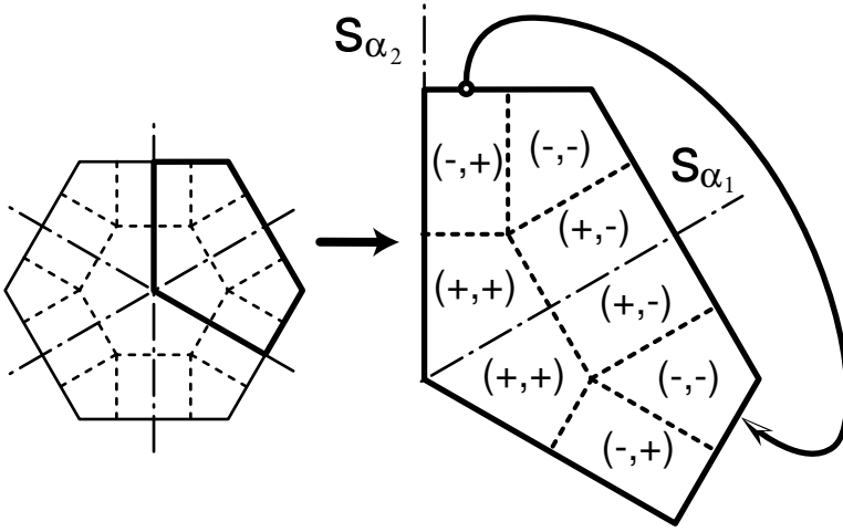
Figure 5. Gluing creates a Mobius band out of two contiguous chambers.
