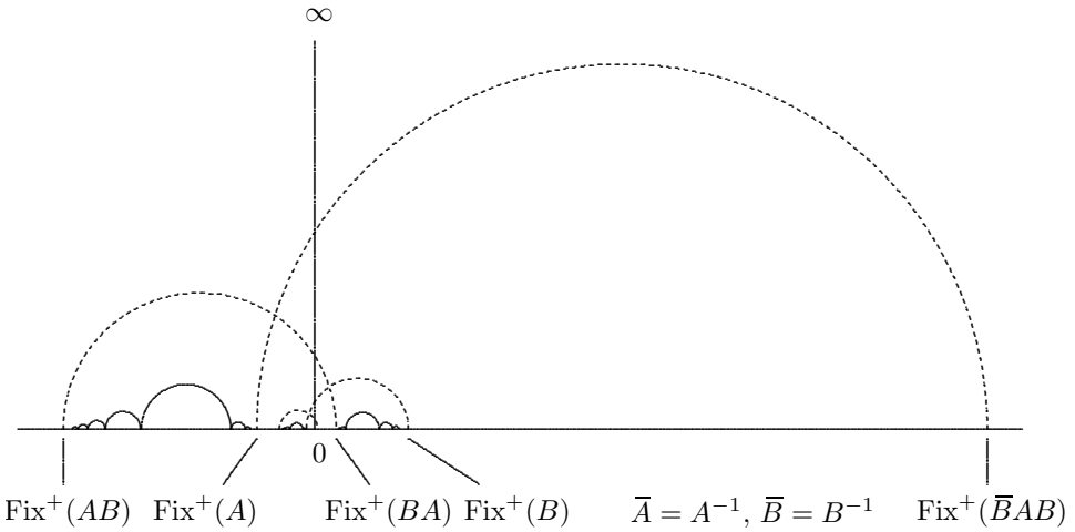
Figure 2. Gaps for M_1 .
