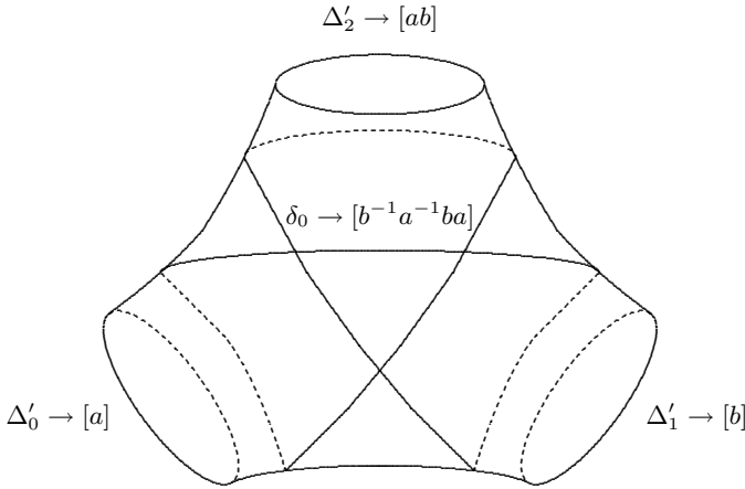
Figure 1. A commutator curve on M_1 .
