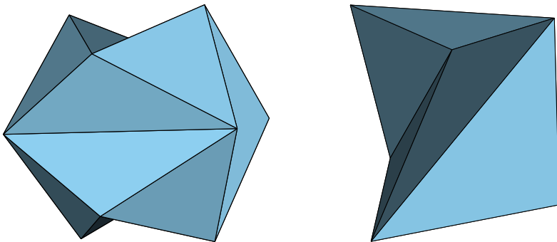
Figure 2. Examples of infinitesimally flexible polyhedra: Jessen's orthogonal icosahedron [ Jessen 1967 ; Weisstein ] and Schönhardt's polyhedron [ Schönhardt 1928 ; Wunderlich 1965 ]. Both examples are weakly convex ( Definition 1.3 ) but not decomposable ( Definition 1.4 ).
