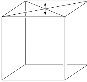
Figure 3. Convex triangulated sphere with a flat vertex. Moving this vertex in the direction orthogonal to the face produces a non-trivial infinitesimal flex.
