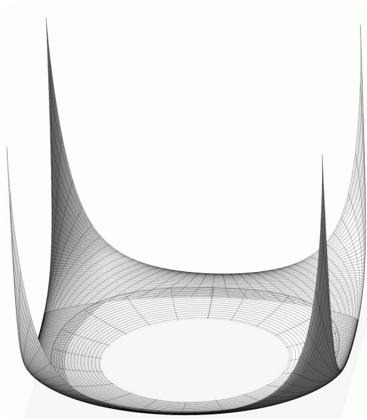
Figure 4. A 2-periodic isocurved surface obtained from Scherk's surface.
