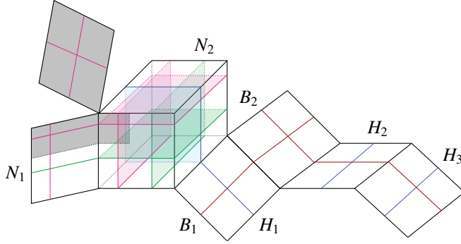
Figure 1. Hyperplanes crossing K (the dark shaded area on the left is \hat{Z} ).
