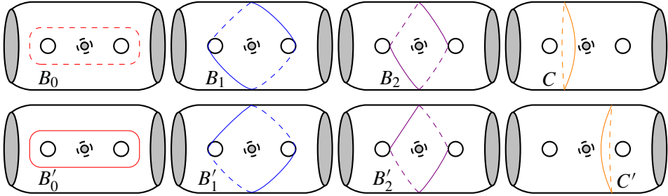
Figure 5. Vanishing cycles of the genus-2 pencil.
