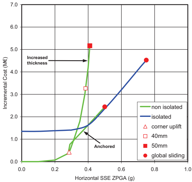
Figure 6. Cost evolution with seismic demand: pile foundation.
