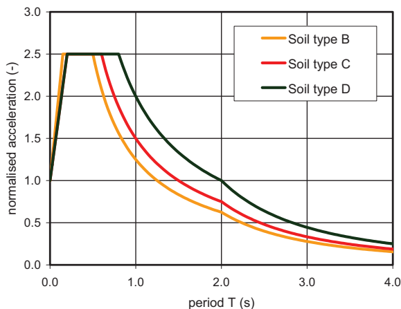
Figure 2. Spectral shapes used in the calculations.
