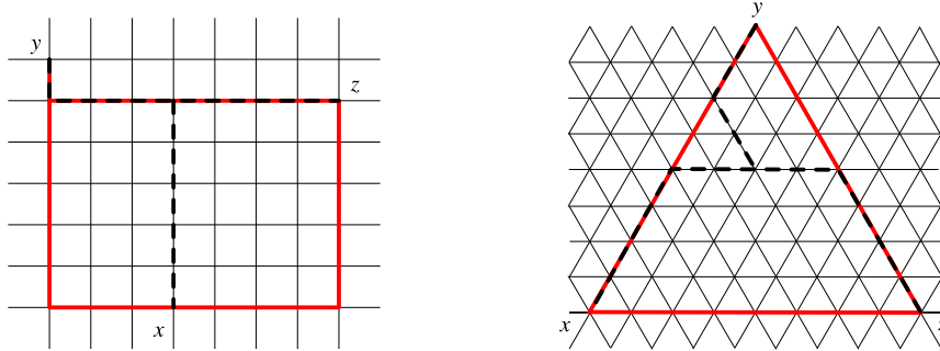
Figure 1: \mathbb{Z}^2 is L_\delta for one generating set and not another
