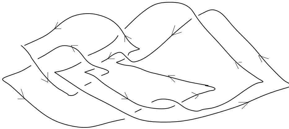
Figure 4: A Legendrian representative of -10_{145}
