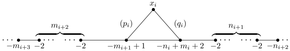
Figure 7: The manifold X^{(i)} for even i
