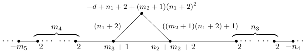
Figure 6: The manifold X^{(2)}
