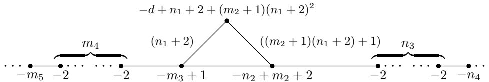
Figure 6: The manifold X^{(2)}
