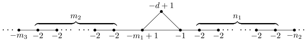
Figure 4: The manifold X^{(0)}
