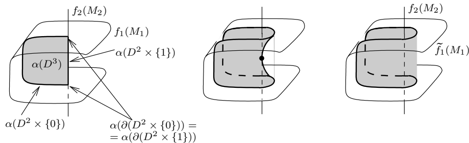
Figure 2: Pushing f_1|_{\beta_\epsilon(D^2 \times I)} across \alpha_\epsilon(D^3 \times I)
