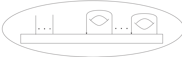
Figure 1: A standard handlebody
