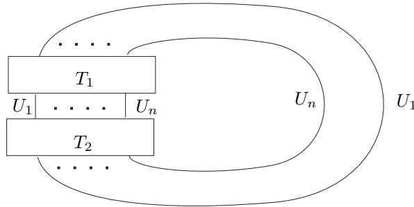
Figure 2: A tangle presentation for \Omega \sqcup L
