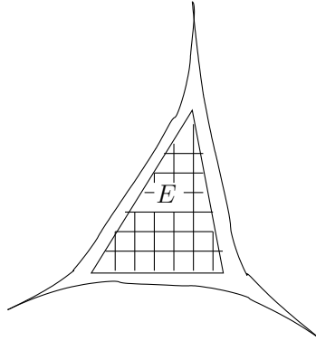
Figure 1: A triangle which is thin relative to the flat E
