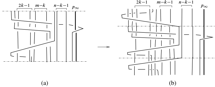
Figure 15: Induction step
