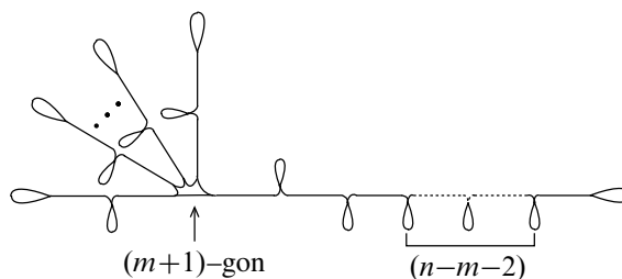
Figure 21: Train track \tau_{\mathfrak{h}_{m,n}}
