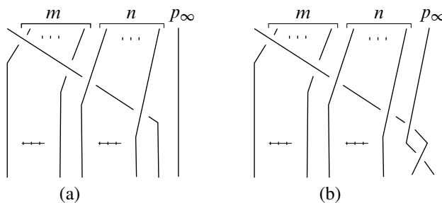
Figure 3: Images of (a) \beta_{m,n} and (b) \sigma_{m,n} in \mathcal{B}(S^2; \mathcal{S}, \{p_\infty\})
