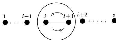
Figure 6: Action of \sigma_i as a homeomorphism of F
