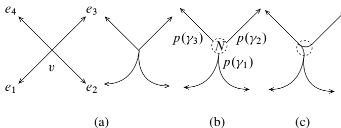
Figure 8: Example of a graph smoothing
