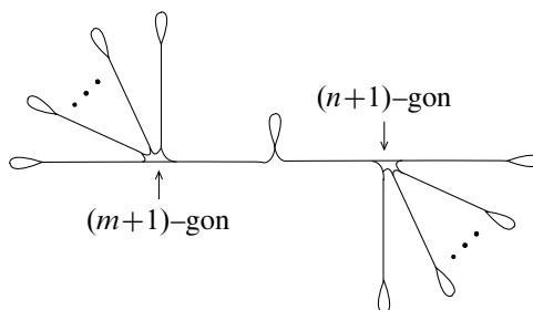
Figure 20: Train track \tau_{\mathfrak{g}_{m,n}}
