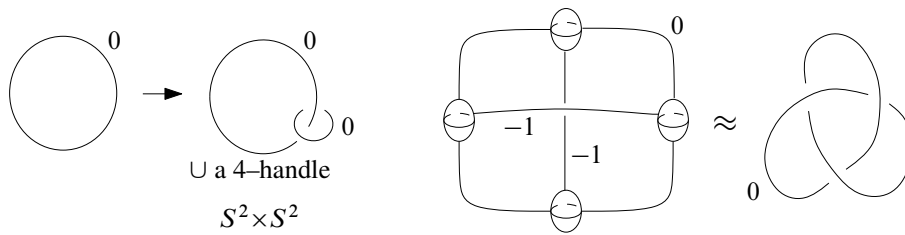
Figure 1: On the left: 0–surgery along the binding yields a trivial S^2 fibration over D^2 on each piece, which make up S^2 \times S^2 . On the right: 0–surgery along the new binding yields a cusp neighborhood on both sides.
