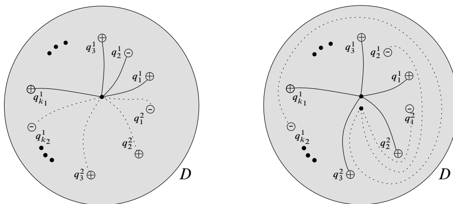
Figure 3: New monodromies from old ones. On the left: \mu_1 is given by solid arcs, and \mu_2 by dotted ones. On the right: Solid arcs are the positive arcs representing \mu_+ , whereas conjugated dotted arcs are negative , providing a representation of \mu_- after closing the base back to S^2 .
