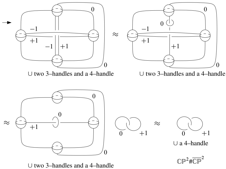
Figure 2: The achiral Lefschetz fibration on the second associated model. The total space is shown to be \mathbb{C}P^2 \# \overline{\mathbb{C}P^2} .
