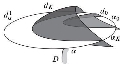
Figure 4: Nested discs intersecting \alpha
