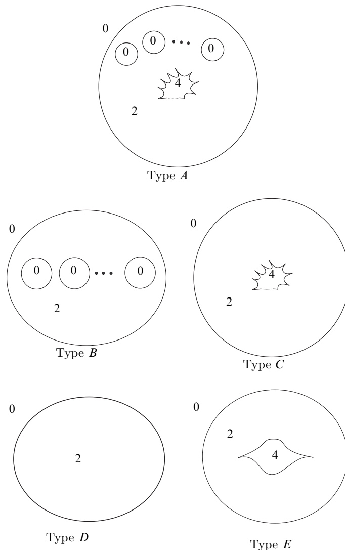
Figure 21: Possible images of the singular set with no fold crossing for F \cong S^2
