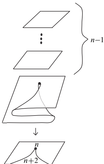
Figure 6: The situation near a cusp
