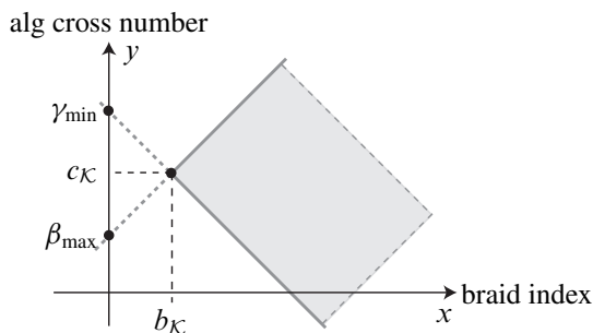
Figure 11: The region of braid representatives of \mathcal{K}
