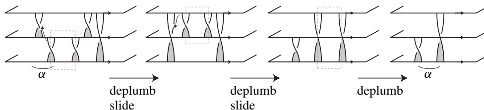
Figure 9: \alpha 123 \rightarrow \alpha
