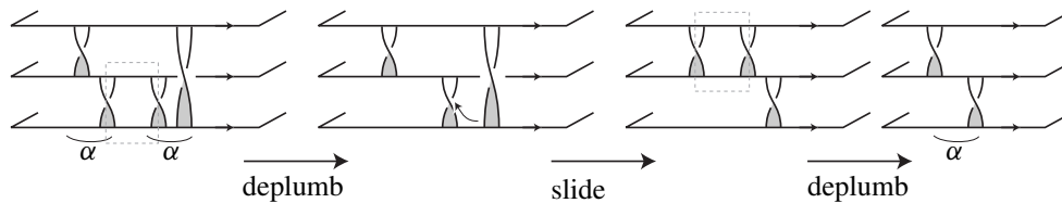
Figure 8: \alpha^2 \rightarrow \alpha
