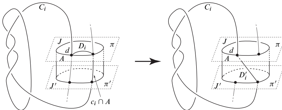
Figure 13: Construction of K_i from \widehat{K}_i
