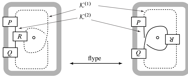
Figure 15: A flype move
