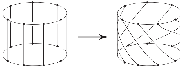
Figure 14: From A \cap \mathbf{K}' to A \cap L , where p = 7, m = 2
