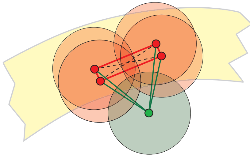
Figure 2: A fake generator for H_2(\mathcal{R}_s, \mathcal{F}_s) which is annihilated by inclusion \iota_* into H_2(\mathcal{R}_w, \mathcal{F}_w) . The strip illustrated is a collar of radius r_f .
