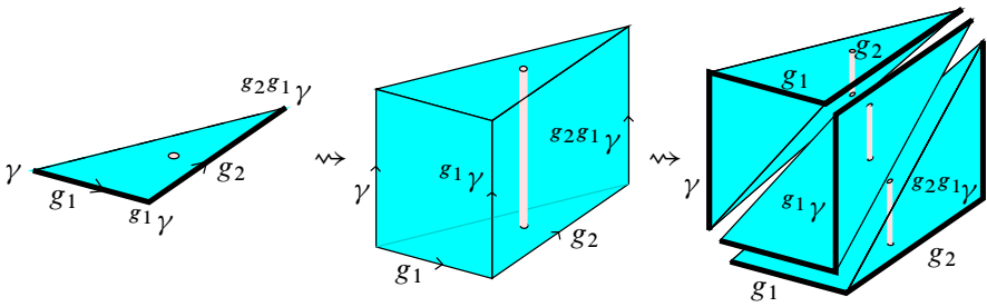
Figure 4: The parmesan construction mapping a point in a two-simplex of B\Lambda\mathcal{G} to a loop in B\mathcal{G} . For reasons of space, here {}^g\gamma denotes g\gamma g^{-1} .
