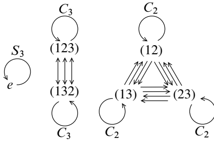
Figure 3: The loop groupoid \Lambda \overline{S_3} or equivalently the action groupoid \mathcal{G}_{S_3}(S_3^c) for S_3 with the conjugation action (where S_3 denotes the symmetric group on three letters). The automorphism groups have been marked on.
