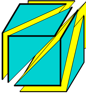
Figure 6: The three-torus decomposed
