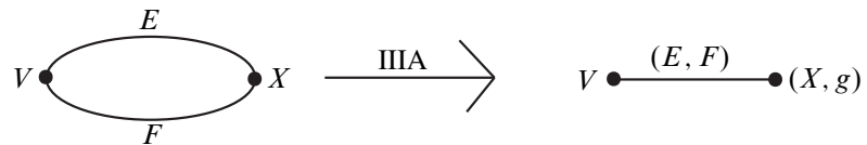
Figure 3: A fold of type IIIA
