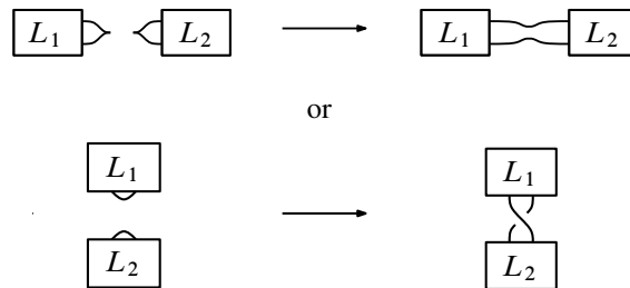
Figure 1: Connected sum of two Legendrian knots
