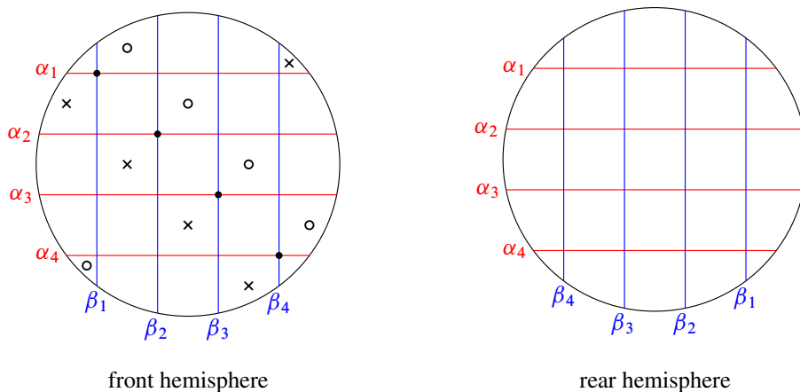
Figure 4: Spherical grid diagram for the trefoil knot
