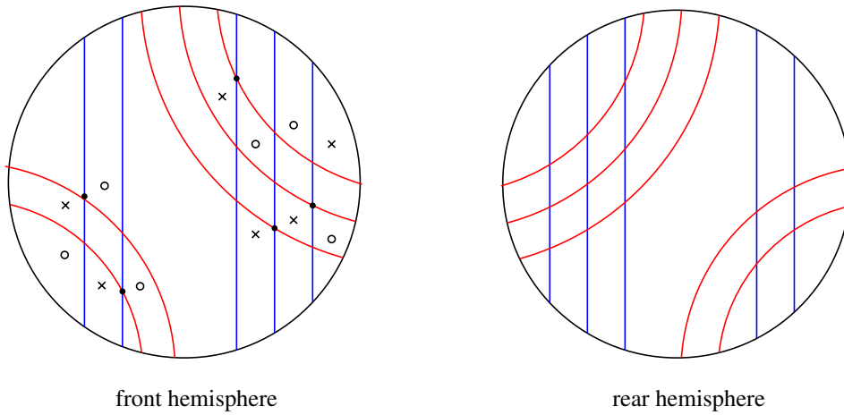
Figure 6: Connected sum
