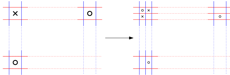
Figure 2: Stabilization of type X:NW
