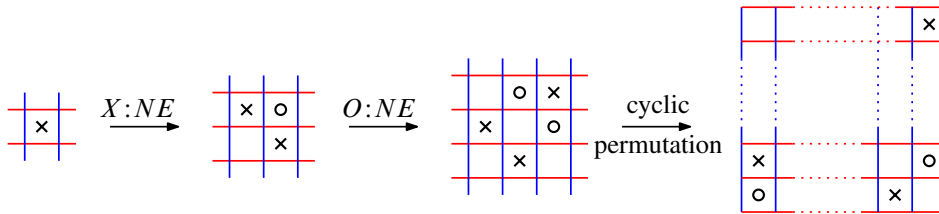
Figure 3: Grid moves
