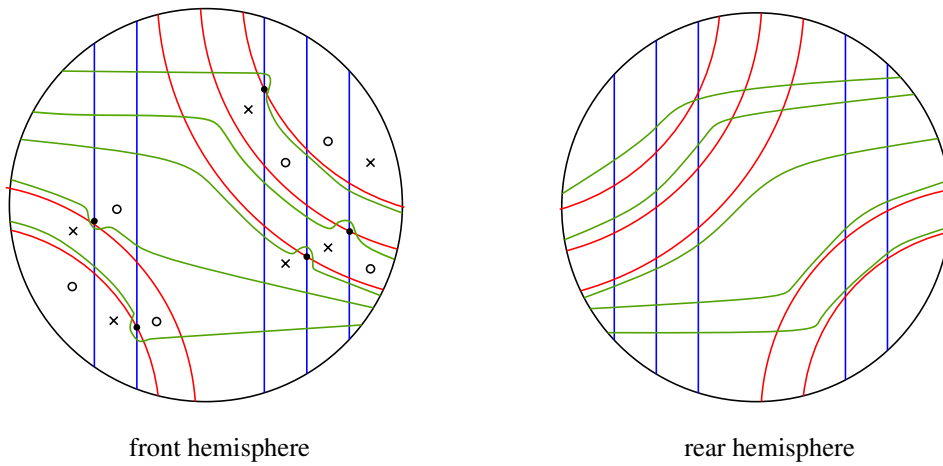
Figure 7: Isotoping to obtain a grid diagram
