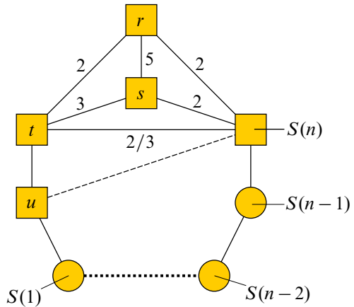
Figure 3. (DE4): n \geq 2 and \overline{X_1 u} = \infty and X_n \subseteq \{r, s, t\}^\infty and r, s, t, u form an H_4 .
