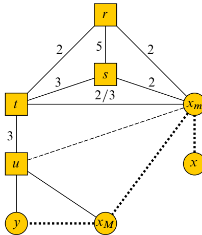
Figure 5. Contradicts (DE4)
