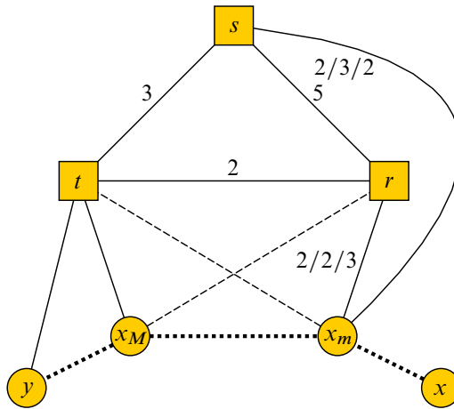
Figure 4. Contradicts (DE3)
