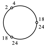
Figure 2: A GBS group with finite labeled graph space and integral modulus
