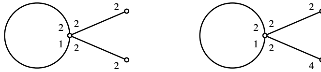
Figure 3: Two nonisomorphic GBS groups
