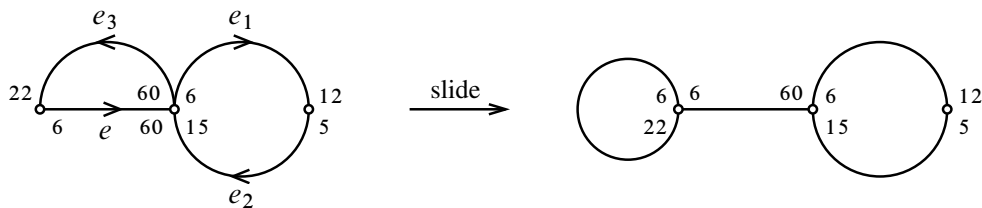
Figure 1: Sliding e_3 over \bar{e} results in a graph with no strict monotone cycles
