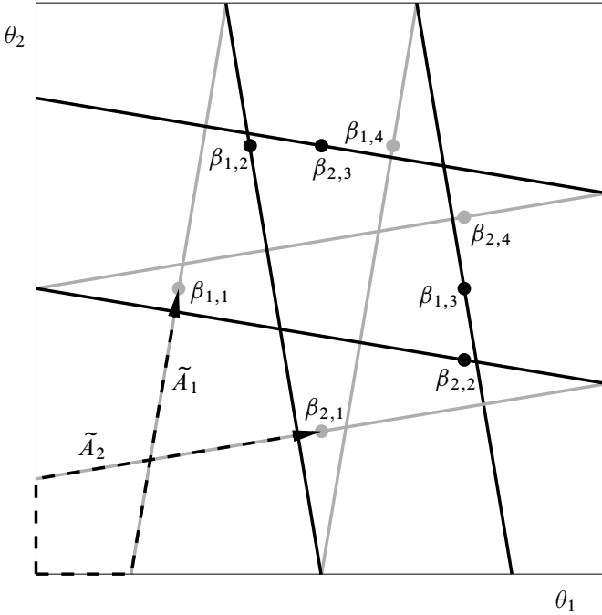
Figure 3: The SU(2) representation varieties of two trefoils
