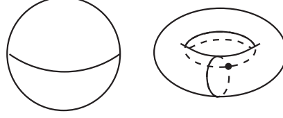
Figure 8: Simple polyhedra of dimension n = 1 (a circle and a trivalent graph) and n = 2 (a sphere and a torus with two discs attached)
