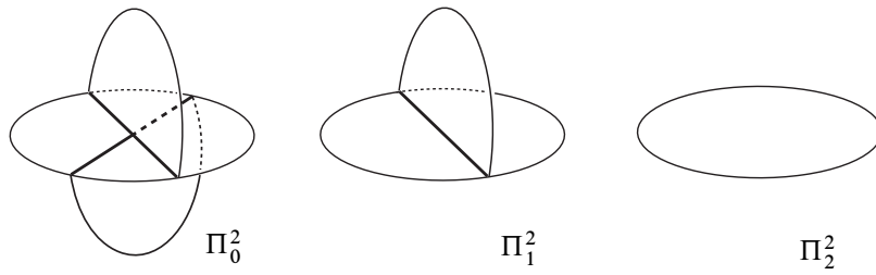
Figure 5: The local models of a simple polyhedron of dimension 2
