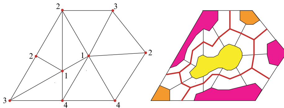
Figure 12: A triangulation T and a partition of the vertices induce a simple polyhedron realized as a subcomplex of T' and some submanifolds M_V realized as subcomplexes of T'' .
