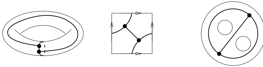
Figure 9: A spine of the torus (left and center) and of the pair-of-pants (right)
