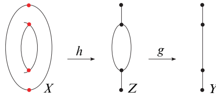
Figure 1: The Stein factorization of a map
