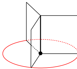
Figure 7: We have \Pi^n \cong (\Pi^{n-1} \times [0, 1]) \cup (D^n \times \{0\}) . Here n = 2 : the disc D^2 \times \{0\} is horizontal and \Pi^1 \times [0, 1] is vertical.
