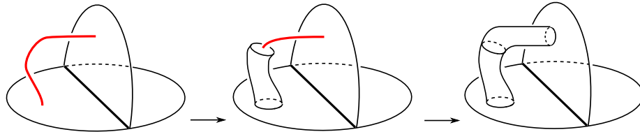
Figure 17: Let Q \cup K be a spine of M , such that Q is simple and \dim K < \dim Q . We obtain a simple spine of M by subdividing K into cells and then drilling them inductively. Each drilling produces a new ball in the complement. Here, K is an arc subdivided into two 1-cells.
