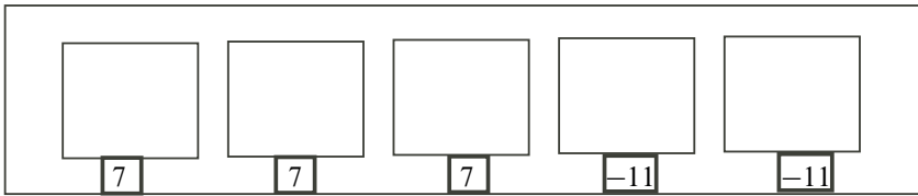
Figure 2: Schematic diagram for 3T_{2,7} - 2T_{2,11}
