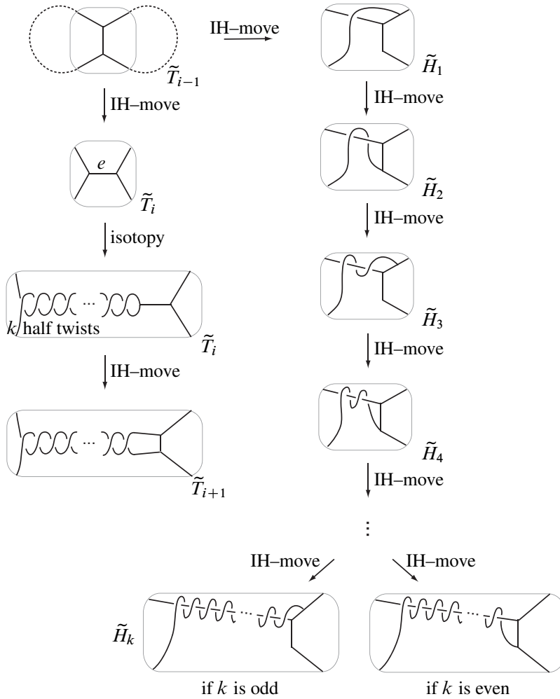
Figure 13: Bypass of sequences of IH-moves
