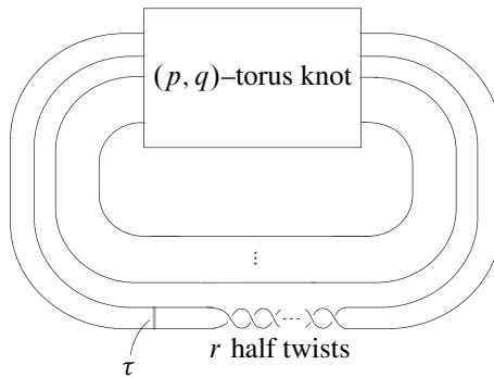
Figure 9: Twisted torus knots K(p, q; r)
