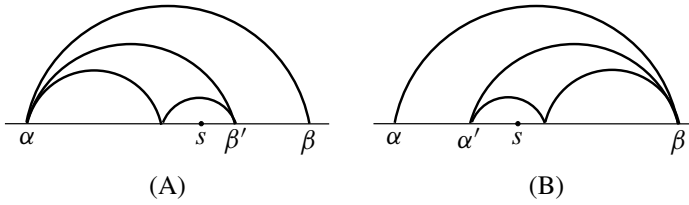
Figure 4: The configurations of Farey arcs of Lemma 2.3
