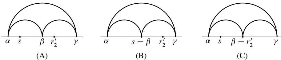
Figure 3: The configurations of Farey arcs of Lemma 2.2
