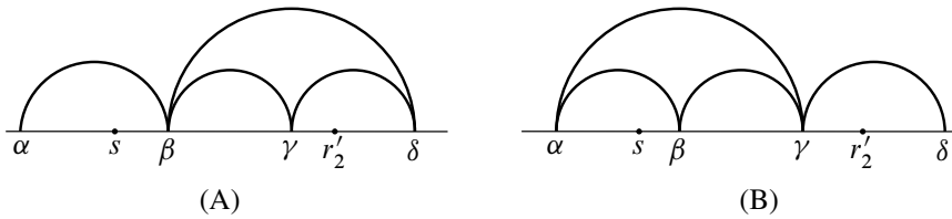
Figure 5: The configurations of Farey arcs of Lemma 2.4
