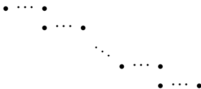
Figure 7: The point diagram underlying Riemenschneider’s point rule
