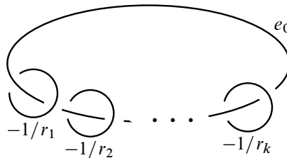
Figure 1: The Seifert 3–manifold Y(e_0; r_1, \dots, r_k)
