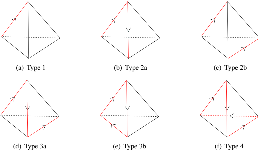
Figure 2: The possibilities for p^{-1}(e) \cap \tilde{\sigma}
