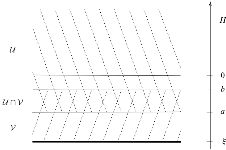
Figure 8: The union W = U \cup V
