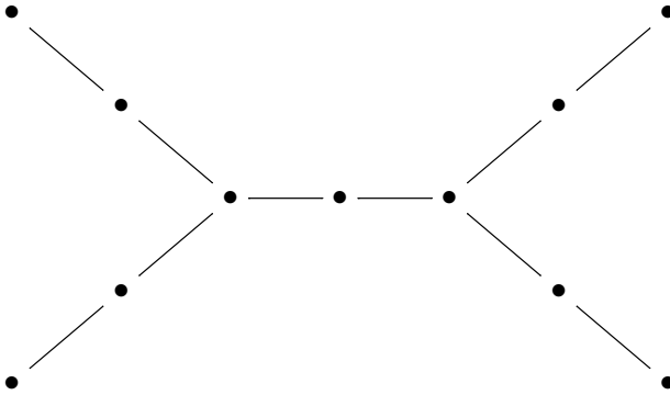
Figure 1: Bass–Serre tree for PSL_2(\mathbb{Z})
