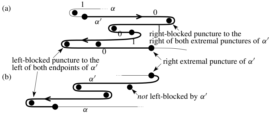
Figure 2: (a) The starting point of \alpha' (the bold line segment) is to the left of the end point. (b) Vice versa.
