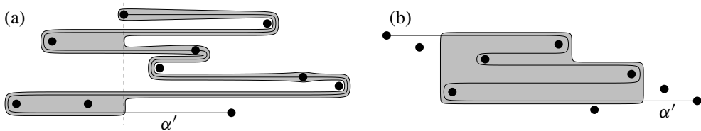
Figure 3: Constructing invariant curves which intersect the curve c . (a) In the case where there is a left blocked puncture to the left of both extremal punctures (b) In the other case.
