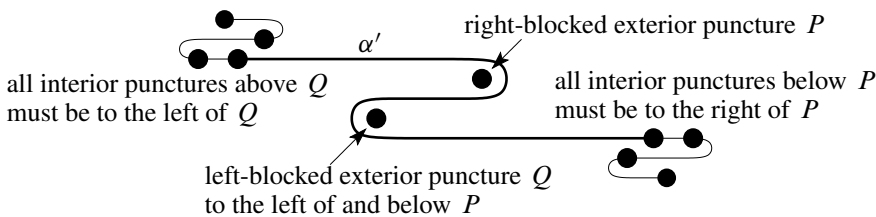
Figure 4: The arc \alpha and (bold) its subarc \alpha'
