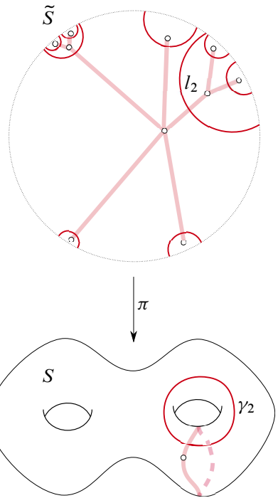
Figure 2. Schematic picture: \pi^{-1}(\gamma_2) , the union of l_2 and all its translates, is a collection of disjoint lines. S - \gamma_2 has only one region, so the dual tree to \pi^{-1}(\gamma_2) has only one orbit of vertices. The action of the fundamental group of S on the tree gives an HNN extension.
