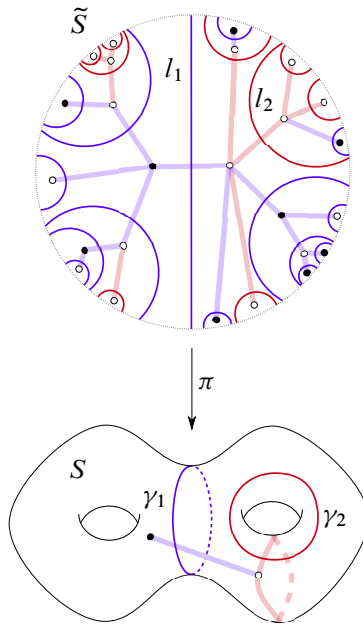
Figure 3. Schematic picture: \pi^{-1}(\gamma_1 \cup \gamma_2) , the union of l_1 , l_2 , and all their translates, is a collection of distinct lines, each projecting to either \gamma_1 or \gamma_2 . Correspondingly, the dual tree to \pi^{-1}(\gamma_1 \cup \gamma_2) has two orbits of edges. The complement S - \pi^{-1}(\gamma_1 \cup \gamma_2) has two types of components: those that project to the left of \gamma_1 , and those that project to the right of \gamma_1 . Correspondingly, the dual tree to \pi^{-1}(\gamma_1 \cup \gamma_2) has two orbits of vertices. This tree is a compatibility tree for the splittings.
