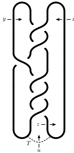
Figure 1: The two-bridge knot 6_2 = K(11, 4) with continued fractions [2, 1, 3] and its associated unknotting tunnel T
