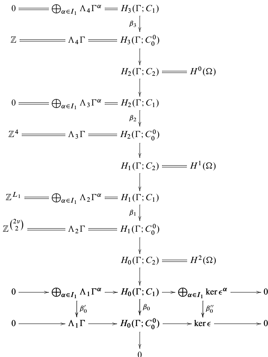
Diagram 5.1: The entire computation for the case \nu = 2 , that is, codimension = dimension = 2 can be summarized in the above diagram in which all rows and columns are exact
