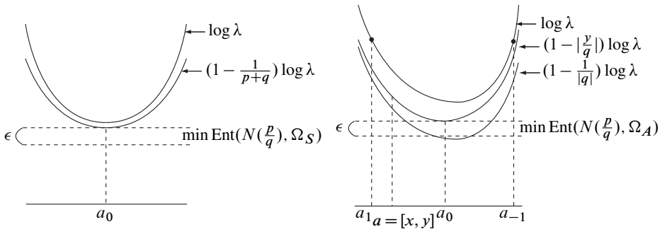
Figure 10: \log \lambda and (1 - 1/(p + q)) \log \lambda on \text{int}(\Delta) \cap S_\gamma(\frac{p}{q}) (left); \log \lambda , (1 - |y/q|) \log \lambda and (1 - 1/|q|) \log \lambda on \text{int}(\Delta) \cap S_\beta(\frac{p}{q}) (right).
