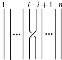
Figure 12: Braid \sigma_i \in B_n
