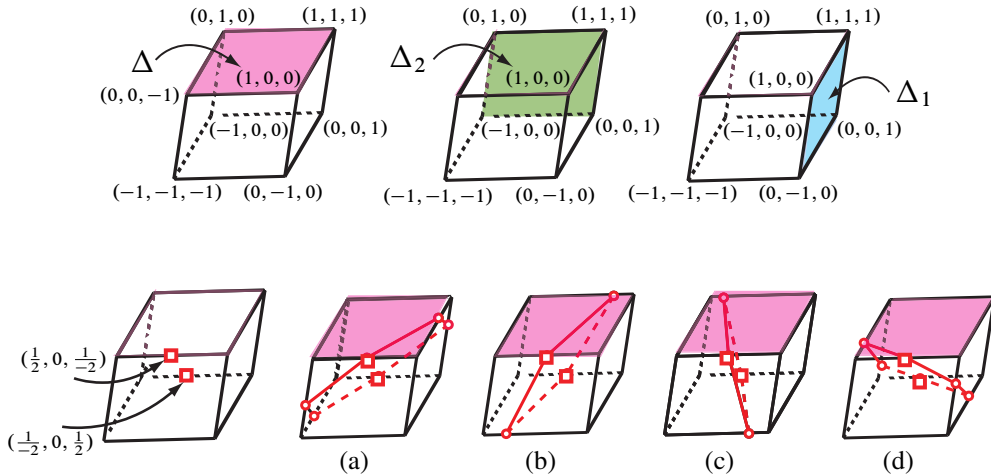
Figure 6: (Top) fibered faces \Delta , \Delta_2 and \Delta_1 , (bottom) \widehat{B}_{\beta,r}(1) in the case (a) r \in (-\infty, -2) , (b) r \in (-2, -1) , (c) r \in (-1, 0) , (d) r \in (0, \infty)
