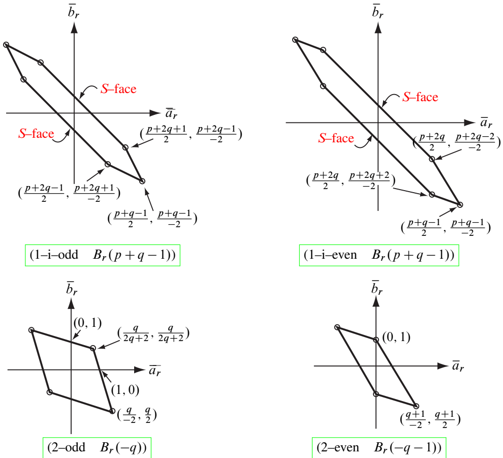
Figure 8: Thurston norm ball B_r(d) (with radius d ) of N(\frac{p}{q}) ; (1-i-odd) p/q \in (-\infty, -2) , q \neq 1 and p is odd; (1-i-even) p/q \in (-\infty, -2) , q \neq 1 and p is even; (2-odd) p/q \in (-2, 0) and p is odd; (2-even) p/q \in (-2, 0) and p is even
