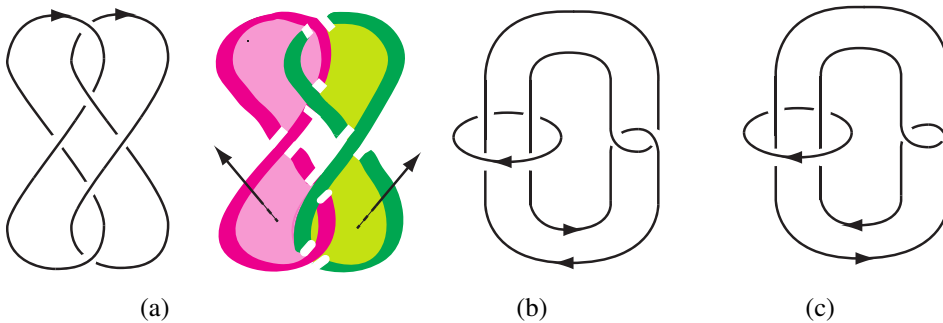
Figure 11: Projections of the Whitehead link [the minimal representatives of \bar{a}_1 and \bar{b}_1 are illustrated in (a)]
