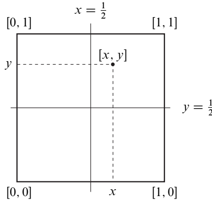
Figure 3: [x, y] \in \text{int}(\Delta)
