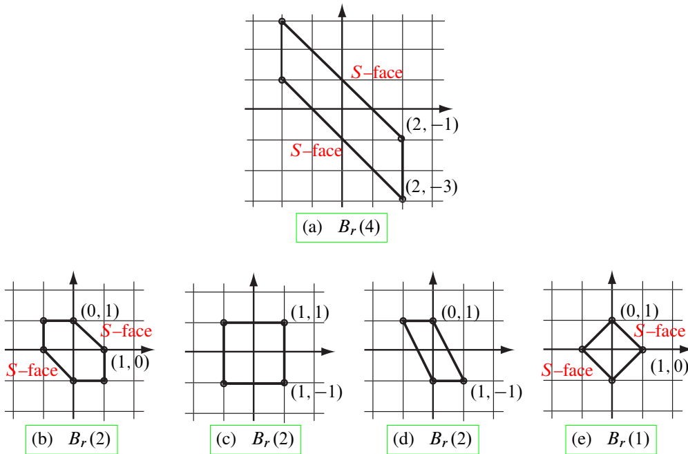
Figure 9: Thurston norm ball B_r(d) (with radius d ) of N(r) when (a) r = -6, 4 , (b) r = \frac{5}{2}, \frac{1}{2} , (c) r = \frac{3}{2}, \frac{1}{2} , (d) r = \frac{4}{3}, \frac{2}{3} , (e) r = 1 .
