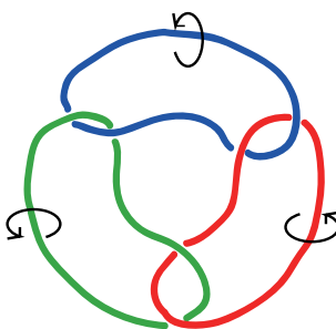
Figure 5: Meridians of the components of C_3
