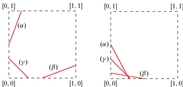
Figure 15: (Left) t/u \in (-\infty, -1) , (right) t/u \in (-1, \infty) [(\alpha) := \text{int}(\Delta) \cap S_\alpha(\frac{t}{u}), (\beta) := \text{int}(\Delta) \cap S_\beta(\frac{t}{u}), (\gamma) := \text{int}(\Delta) \cap S_\gamma(\frac{p}{q})]
