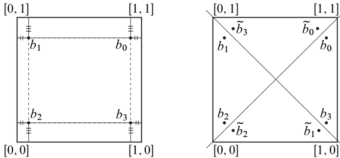
Figure 4: We have that b_0 = [\frac{x}{x+y-z}, \frac{y}{x+y-z}] , b_1 = [\frac{y-z}{x+y-z}, \frac{y}{x+y-z}] , b_2 = [\frac{y-z}{x+y-z}, \frac{x-z}{x+y-z}] , b_3 = [\frac{x}{x+y-z}, \frac{x-z}{x+y-z}] \in \text{int}(\Delta) and \tilde{b}_i \in \text{int}(\Delta)
