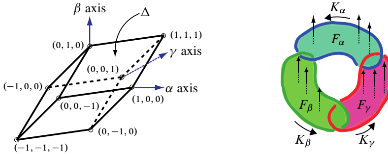
Figure 2: (left) Thurston norm ball for N , (right) F_\alpha, F_\beta, F_\gamma [arrows indicate the normal direction of oriented surfaces]
