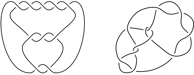
Figure 1: On the left, the (5, -3, 2) -pretzel knot (aka 10_{125} ), the smallest knot with s_3 \neq s_2 ; on the right (drawn with knotscape [13]), 12n_{340} , the smallest knot with |s_3| > |s_2|
