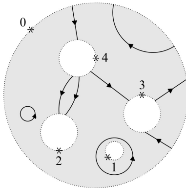
Figure 2: Example of an input diagram (also called spaghetti-and-meatballs diagram) with boundary labelling (+ - + - +, \emptyset, ++, ++-, + - - -)
