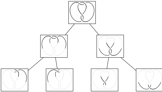
Figure 6: Example of a sub-tangle tree of the figure-eight-knot with girth 4
