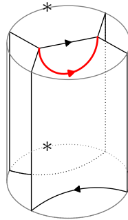
Figure 4: A singular saddle is the intersection of a closed theta foam (not drawn) with a can (drawn grey). It has three facets, one singular edge and degree 1. Orientations and base-points of the domain and codomain are specified.
