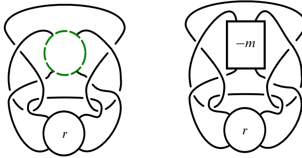
Figure 13: The tangle \mathcal{S}_r^- and the link L_{m,r}^-
