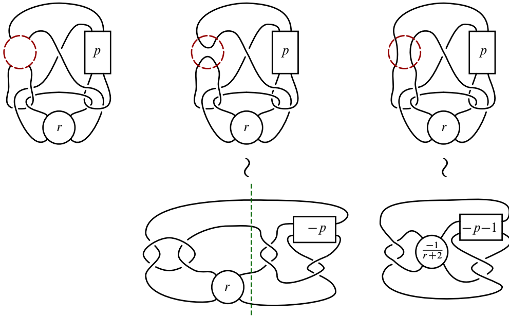
Figure 10: The tangle \mathcal{S}_{p,r} , along with two fillings, \mathcal{S}_{p,r}(0) and \mathcal{S}_{p,r}(\infty) , and their equivalents after isotopy
