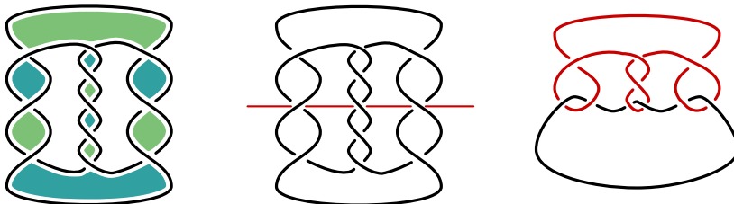
Figure 18: (a) The knot P(3, -3, 2m + 1) (here, m = -3 ), shown as the boundary of a punctured torus, (b) along with the axis of the cycle f of period 2 of the knot and (c) the quotient knot K_f (here, the unknot), along with the image of \text{Fix}(f) in the quotient.
