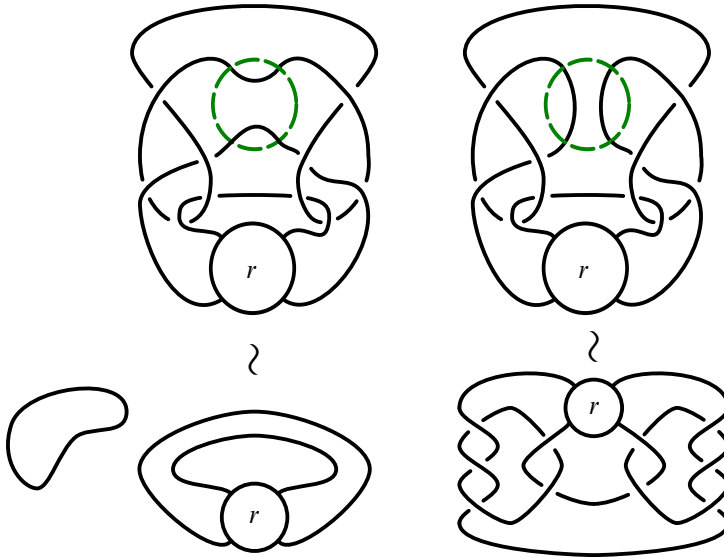
Figure 14: Two interesting fillings of S_r^-
