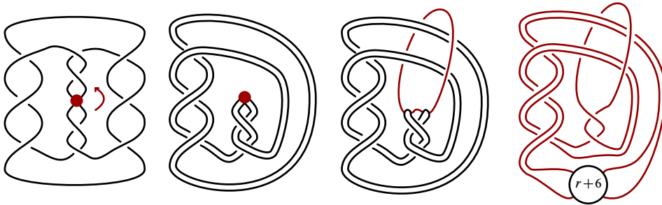
Figure 16: The figures above illustrate how to obtain the quotient tangle \mathcal{T}_m by applying the Montesinos trick to the strong inversion of P(3, 3, 2m + 1) given by rotating the knot \pi radians through its center. Here, m = -3 .
