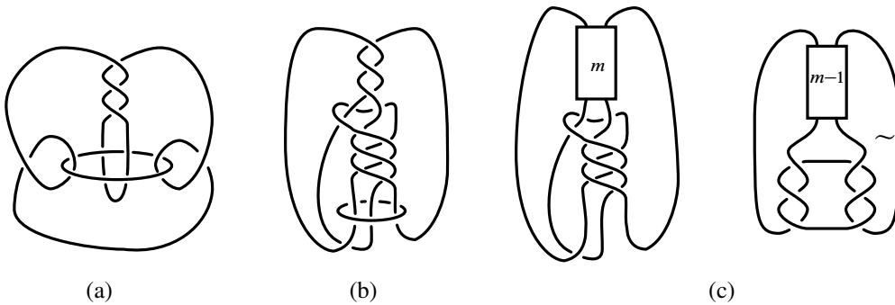
Figure 21: (a) The link (K_m)_f \cup \text{Fix}(f) in the quotient, (b) the link (L_m)_f resulting from 1–surgery on the unknotted component (note that the core of the surgery torus is a component of the resulting link) and (c) the tangle formed by removing the m –twist area of the knotted component J_m of the resulting link. Here, m = -3 .
