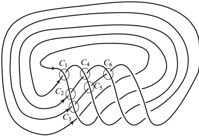
Figure 6: Minimal U -crossing data for T(5, 4)
