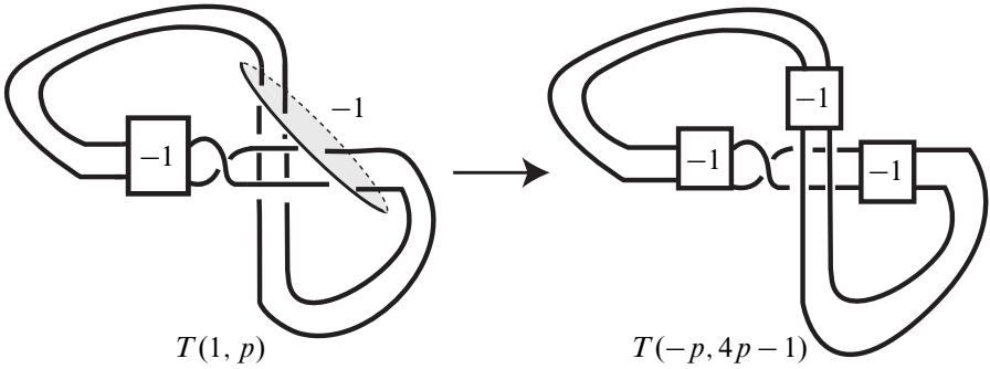
Figure 2: T(1, p) \cong U \xrightarrow{(-1, 2p)} T(-p, 4p - 1)
