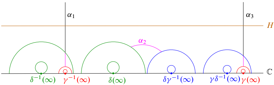
Figure 3: Lifts of g consists of the arcs \alpha_1 , \alpha_2 , and \alpha_3
