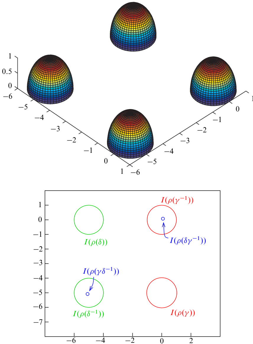
Figure 2: Isometric spheres from Example 2.13 are shown in 3-dimensions at the top and their 2-dimensional intersections with \mathbb{C} at the bottom
