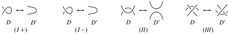
Figure 2: Reidemeister moves
