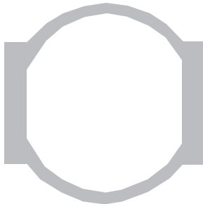
Figure 9: Recovering a circle from a rough pixelation
