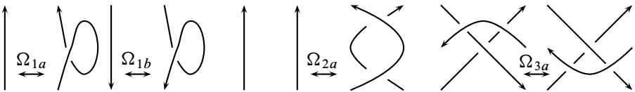
Figure 3: Reidemeister moves
