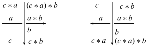
Figure 11: Shadow coloring at a crossing
