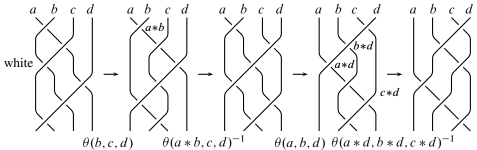
Figure 8: Right-hand side of the tetrahedral move
