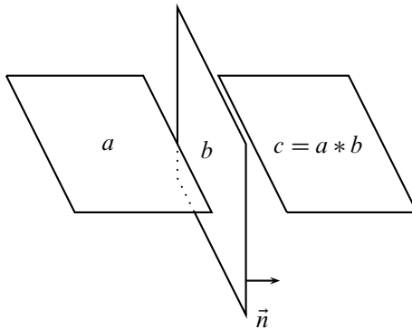
Figure 5: Coloring rules at a double curve
