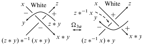
Figure 4: Proper colorings under \Omega_{3a}
