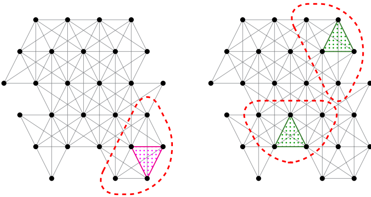
Figure 22: Examples of 4-reductions of the type [a, b, c, de]
