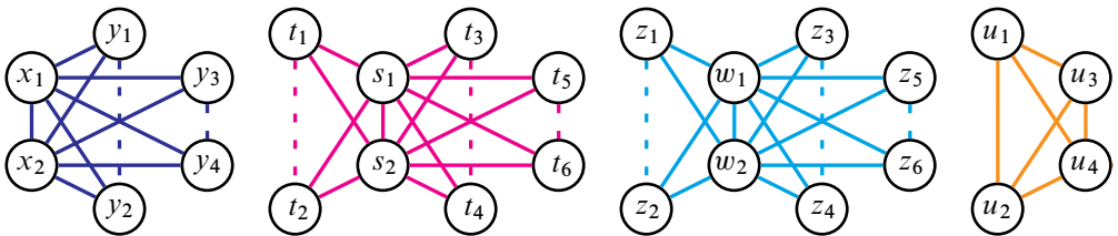
Figure 35: A graph representing \pi_1 of the products of surfaces necessary for this 4-manifold construction
