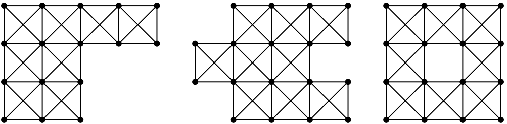
Figure 11: Examples of graphs in the grid family
