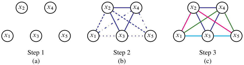
Figure 7: A graph showing the path of edges created by the 4-reduction [x_1x_5, x_2, x_3, x_4]
