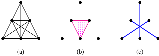
Figure 21: (a) The edges eventually created by a 4–reduction of type [a, b, c, def] , (b) the triangle created by a, b and c , and (c) the edges belonging to the maximal isotropic subspace
