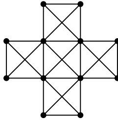
Figure 10: The defining graph for \pi_1 of the manifold described in Lemma 5.7
