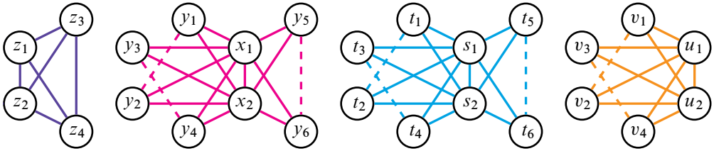
Figure 38: A graph representing \pi_1 of the products of surfaces necessary for this 4–manifold construction
