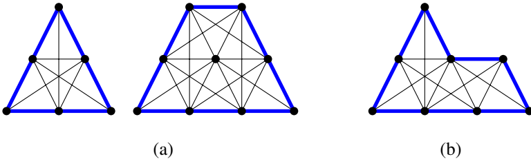
Figure 17: The graphs in (a) are thick and the graph in (b) is thin .
