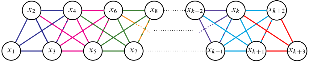
Figure 14: The graph of \pi_1 of the realizing 4-manifold when k is even
