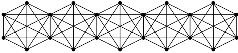
Figure 34: A graph of 6-cliques attached edge-to-edge
