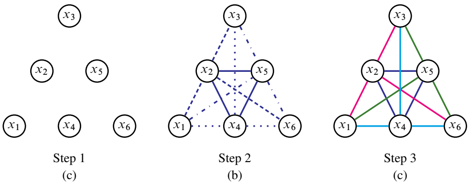
Figure 8: A graph showing the path of edges created by the 4–reduction [x_1x_3x_6, x_2, x_4, x_5]
