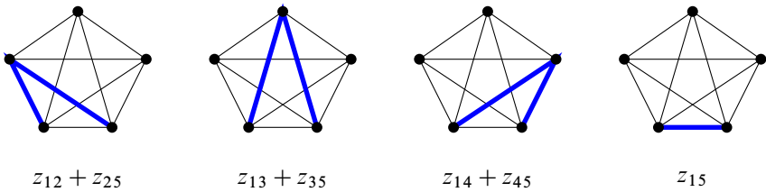
Figure 28: 4 basis elements in the radical for k = 1 and \alpha = s_{1234} + s_{2345}
