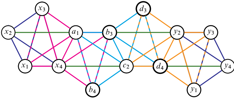
Figure 33: A graph representing \pi_1 of a realizing manifold for four 5-cliques attached edge-to-edge
