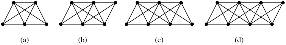
Figure 12: Graphs in the string family
