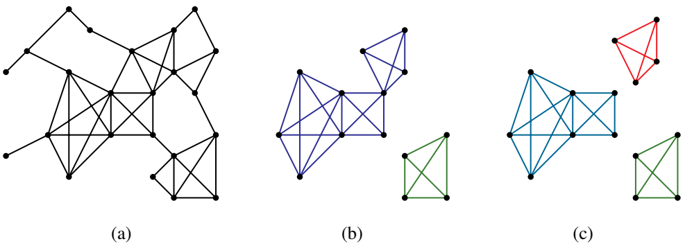
Figure 5: An example of the breakdown of a graph into disjoint subgraphs, for the calculation of h according to Theorems 1.4 and 1.5
