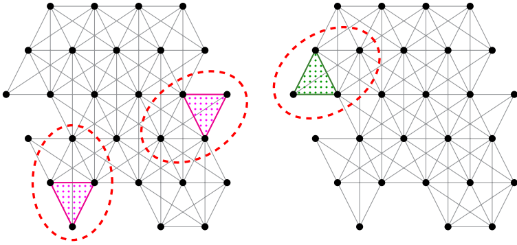
Figure 24: Examples of 4-reductions of the type [a, b, c, d]
