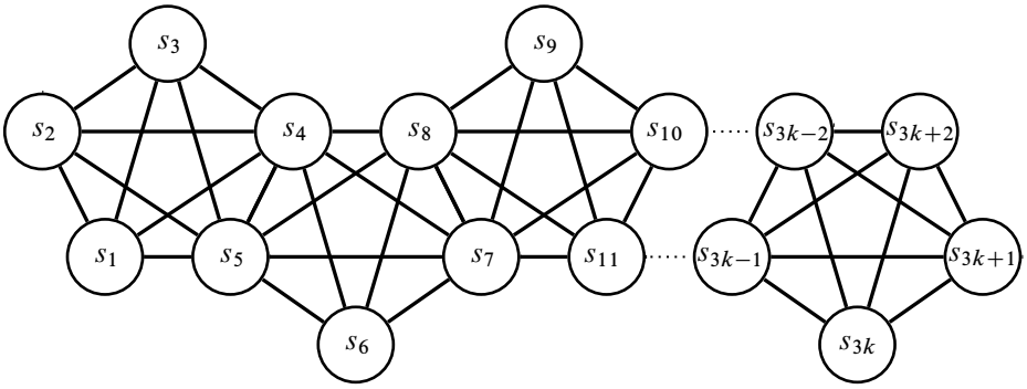
Figure 27: A graph of k 5-cliques attached edge-to-edge
