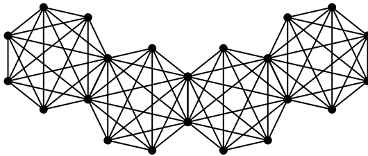
Figure 37: A graph of 7-cliques attached edge-to-edge
