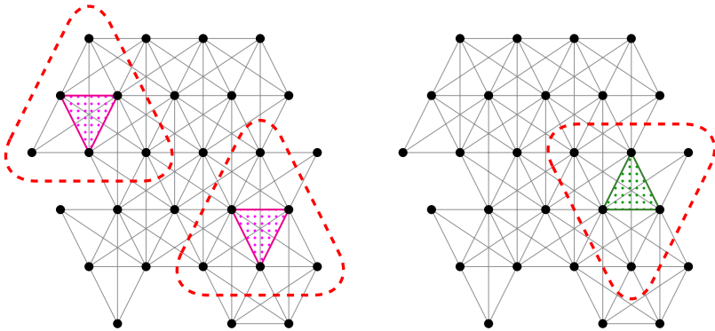
Figure 20: Examples of 4–reductions of the type [a, b, c, def]
