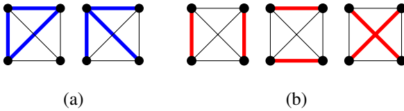
Figure 4: Triangles and claws, formed by the bold edges in (a), are subgraphs that make up an isotropic subspace in each 4-clique. Pairs of edges highlighted in (b) do not.
