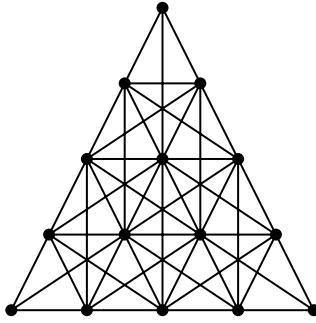
Figure 16: A graph in the hex family
