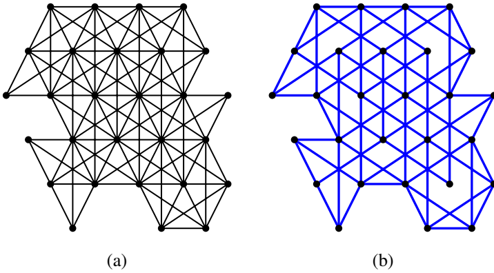
Figure 18: (a) A graph in the hex family as well as (b) the edges that form an isotropic subspace
