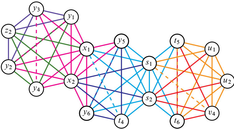
Figure 39: A graph representing \pi_1 of a realizing manifold for three 7-cliques attached edge-to-edge
