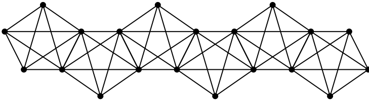
Figure 26: A graph of 5-cliques attached edge-to-edge
