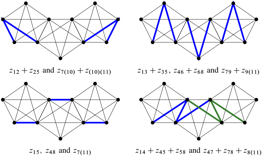
Figure 30: 10 basis elements in the radical for k = 3 and \alpha = s_{1234} + s_{2345} + s_{4567} + s_{5678} + s_{789(10)} + s_{89(10)(11)}
