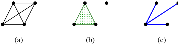
Figure 25: (a) The edges created by a 4-reduction of type [a, b, c, d] , (b) the triangle created by a, b and c , and (c) the edges belonging to the maximal isotropic subspace
