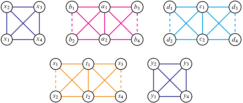
Figure 32: A graph representing \pi_1 of the products of surfaces necessary for this 4-manifold construction
