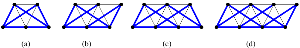
Figure 13: The bold edges of each graph form a maximal isotropic subspace.
