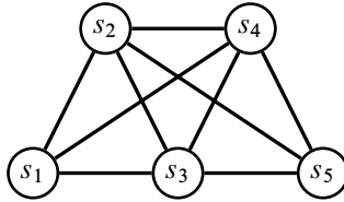
Figure 2: The defining graph \Gamma for G .
