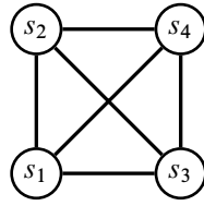
Figure 3: A 4-clique, the defining graph for \mathbb{Z}^4 .
