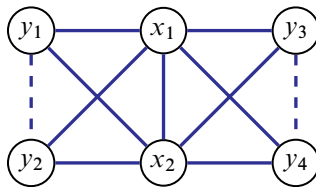
Figure 6: A graph representing \pi_1(T^2 \times \Sigma_2)
