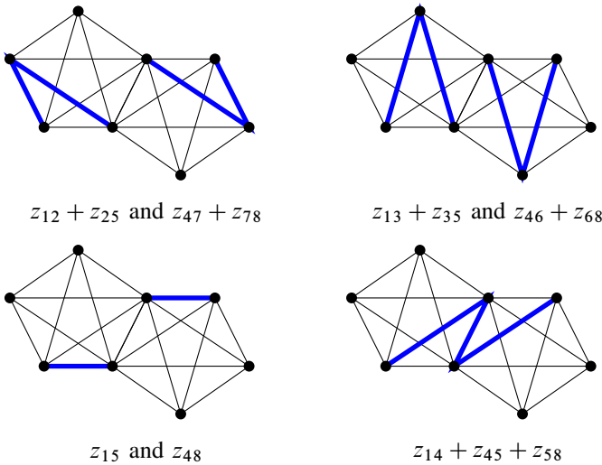
Figure 29: 7 basis elements in the radical for k = 2 and \alpha = s_{1234} + s_{2345} + s_{4567} + s_{5678}
