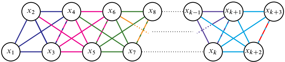
Figure 15: The graph of \pi_1 of the realizing 4-manifold when k is odd
