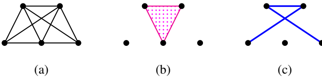
Figure 23: (a) The edges eventually created by a 4-reduction of type [a, b, c, de] , (b) the triangle created by a, b and c , and (c) the edges belonging to the maximal isotropic subspace
