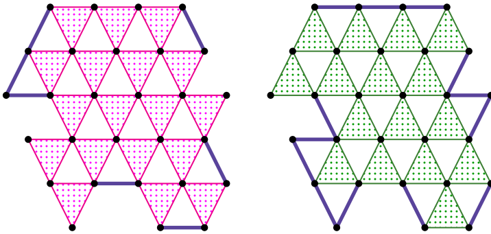
Figure 19: Two constructions for a realizing 4-manifold for a graph in the hex family
