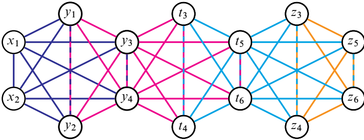
Figure 36: A graph representing \pi_1 of a realizing manifold for three 6-cliques attached edge-to-edge
