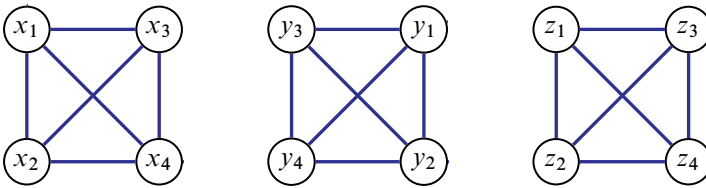
Figure 9: A graph representing \pi_1(T^4 \# T^4 \# T^4)
